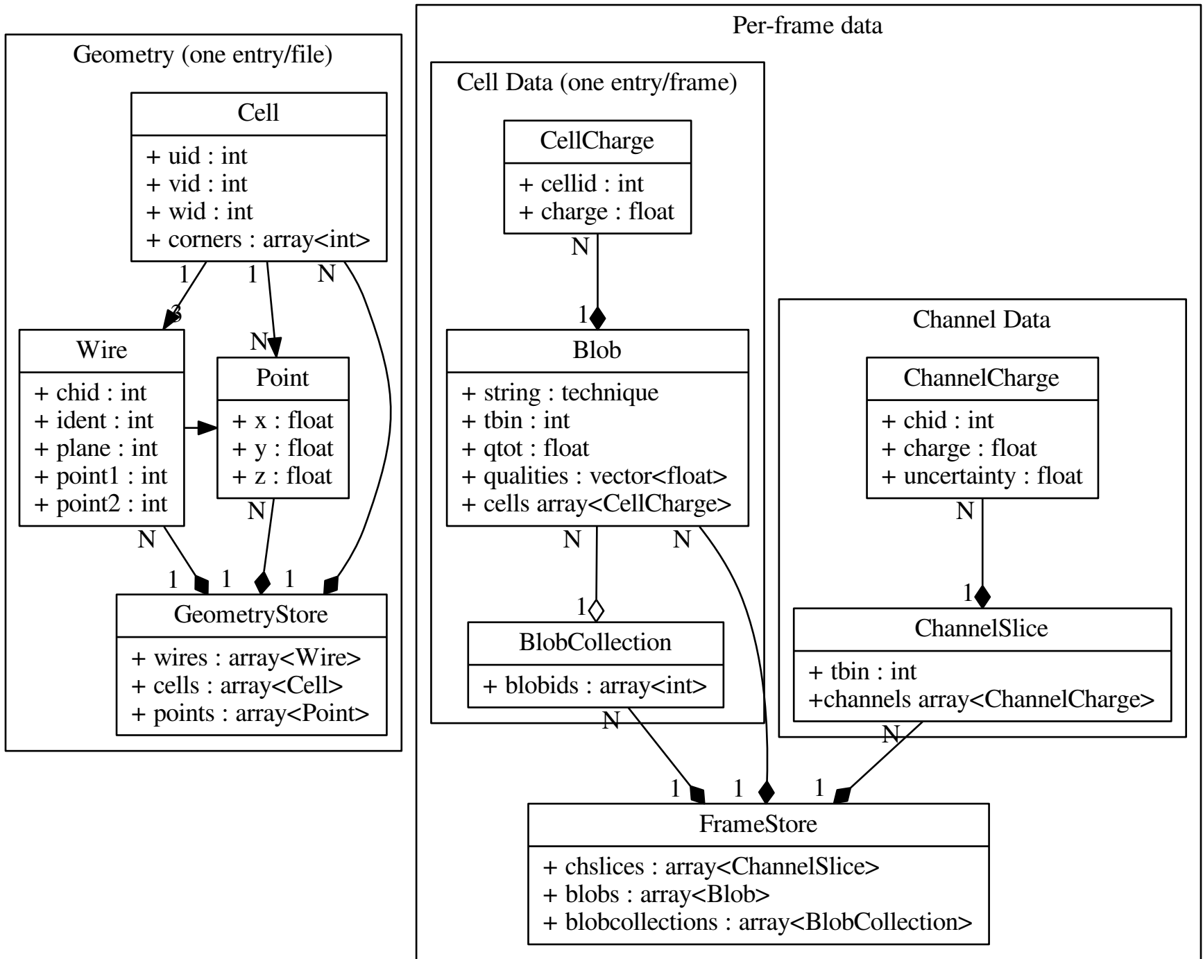
Wire Cell Root Data Schema
